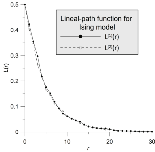
Fig. 6. Lineal-path function for the Ising model microstructure versus distance r given in pixels
