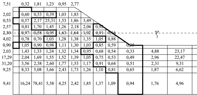
Fig. 5. Factor of safety distribution inside embankment for cyclic load (WTL at 5 m)
