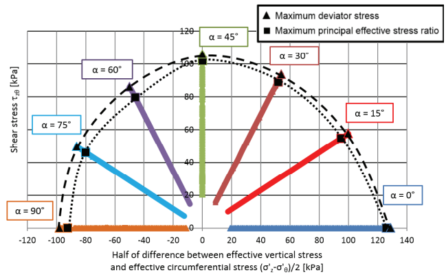
Fig. 2. Effective stress paths for sandy silty clay in axes (\sigma'_z - \sigma'_\theta)/2 - \tau_{z\theta}
