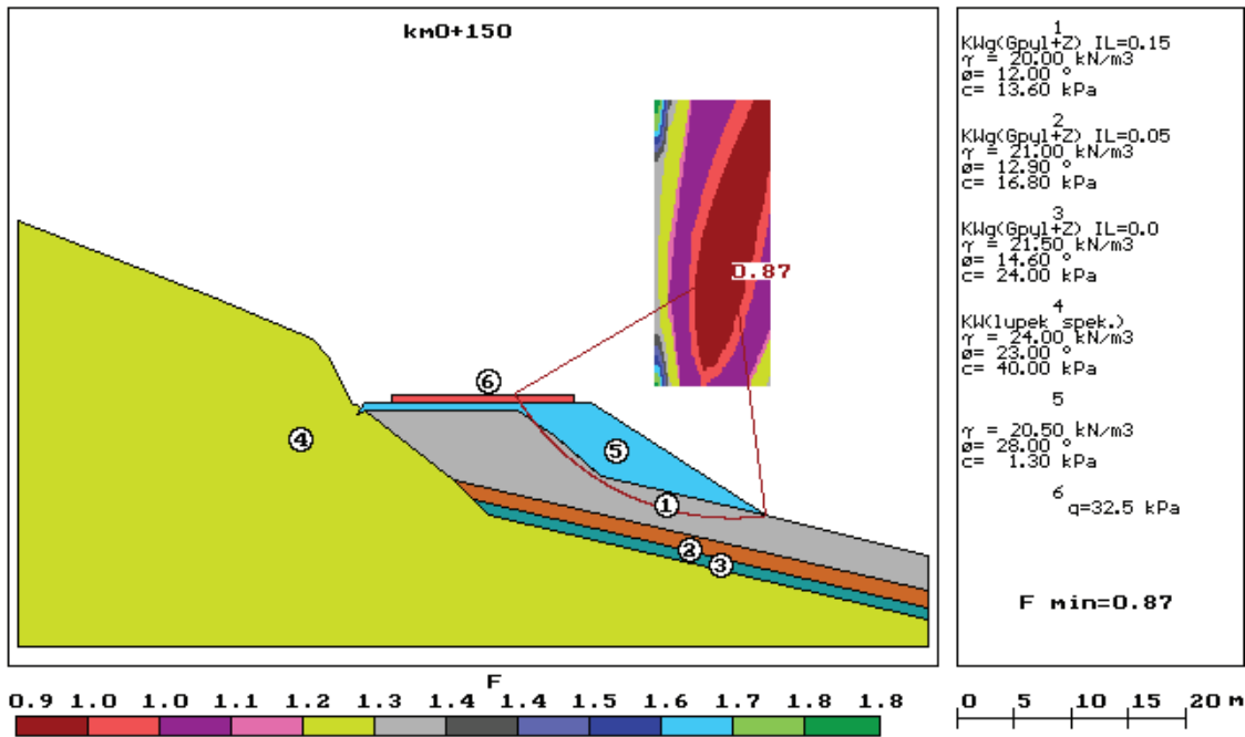
Figure 2: Bolków ring road, cross section of km 0 + 150.02: stability according to EC7 of embankment made of non-cohesive soil.
