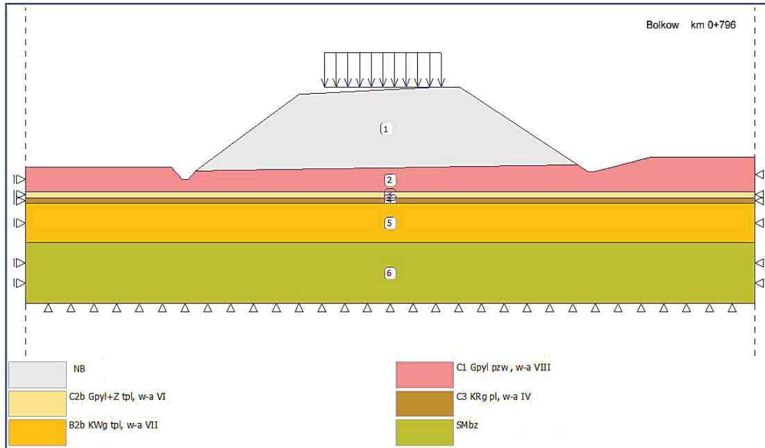
Figure 4: Cross section of km 0 + 796.18 – computational scheme.
