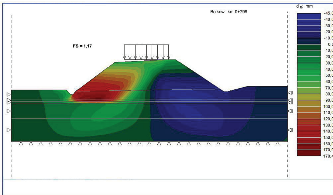
Figure 5: Cross section of km 0 + 796.18 – stability calculations (distribution of displacements) of the embankment made of cohesive soil \gamma = 20.5 \text{ kN/m}^3 , \phi = 17^\circ , c = 22 \text{ kPa} , according to Eurocode 7 ( F_{min} = 1.17 > F_{req} = 1.0 )
