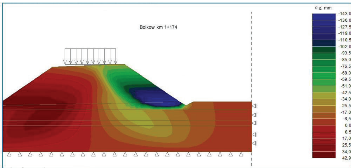
Figure 7: Potential mechanism of the loss of stability – green-blue block in the right slope..
