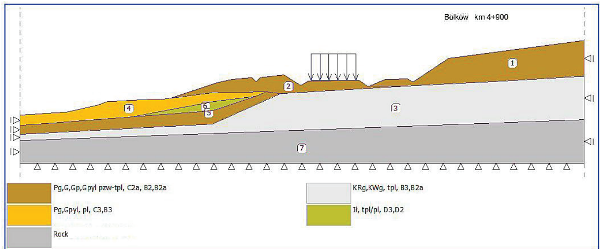
Figure 9: System of ground layers. Phase 2 of calculations – state with road load after the performance of a road excavation
