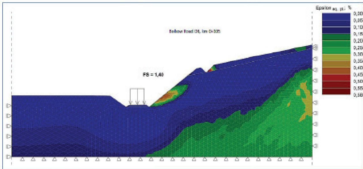
Figure 14: Results of stability calculations of the slope F_{min} = 1.40 .
