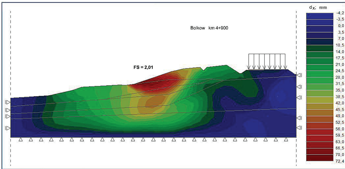
Figure 11: Phase 2 calculations – stability analysis of lower part of the slope below the road excavation F_{min} = 2.01 .
