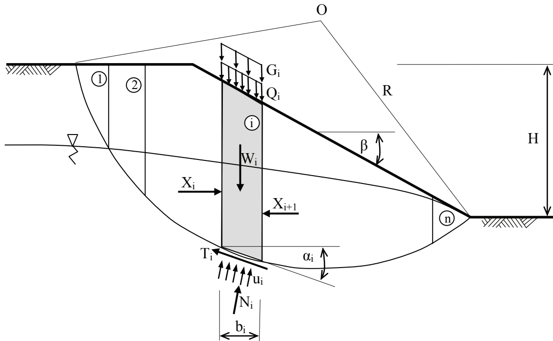
Figure 1: Scheme of the Bishop method (simplified).
