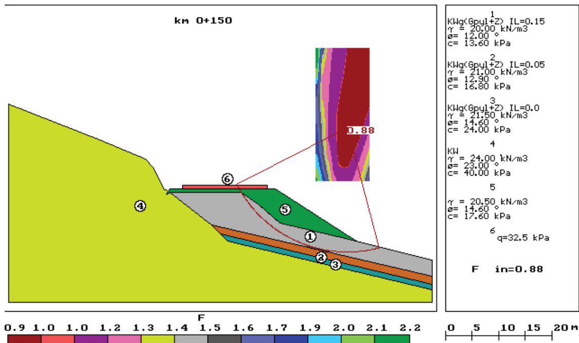
Figure 3: Bolków ring road, cross section of km 0 + 150.02: stability according to EC7 of embankment made of cohesive soil, along with the substrate
