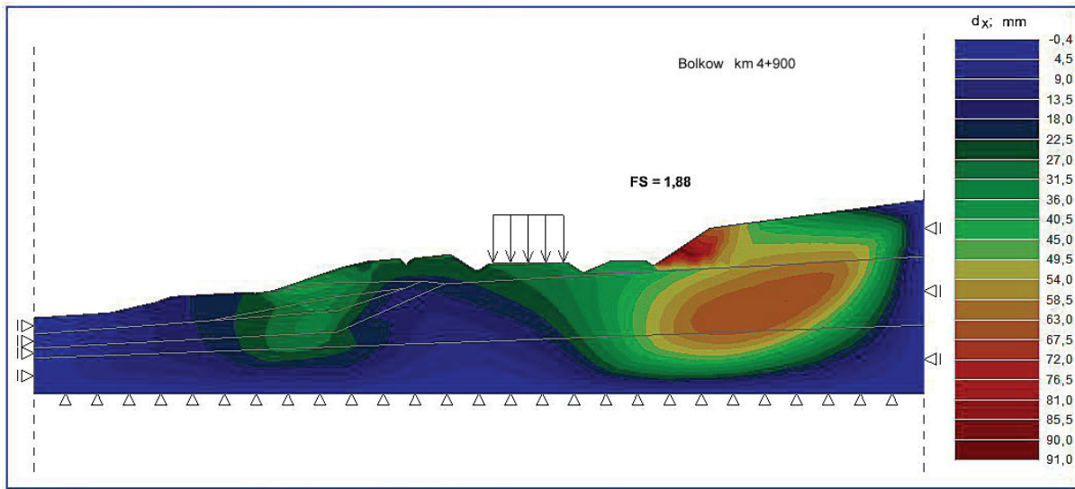
Figure 10: Phase 2 of calculations – stability analysis of the upper part of the slope above the road excavation, F_{min} = 1.88 .
