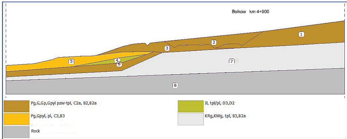
Figure 8: System of ground layers. Phase 1 of calculations – state before performance of a road excavation.
