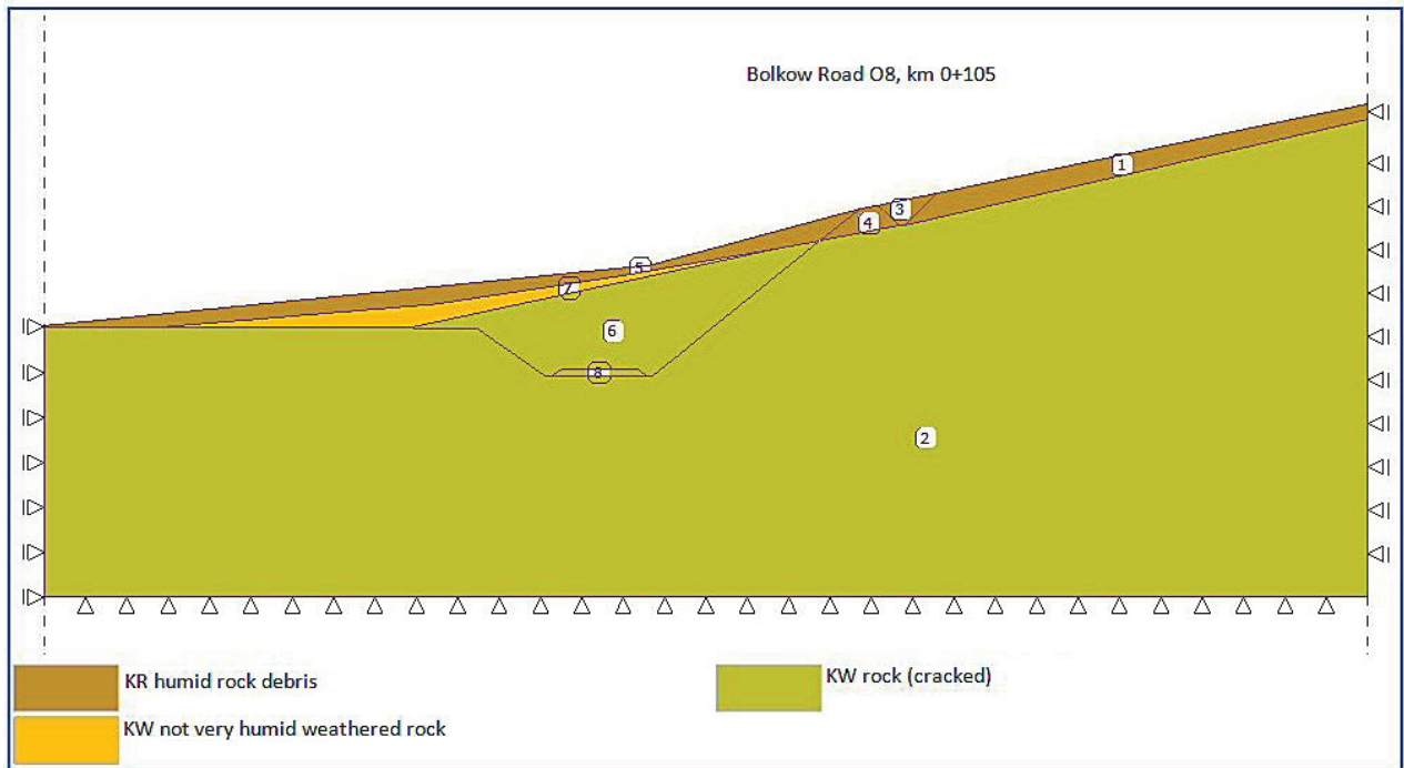
Figure 12: Current profile of the road O8 slope at km 0 + 105.00.
