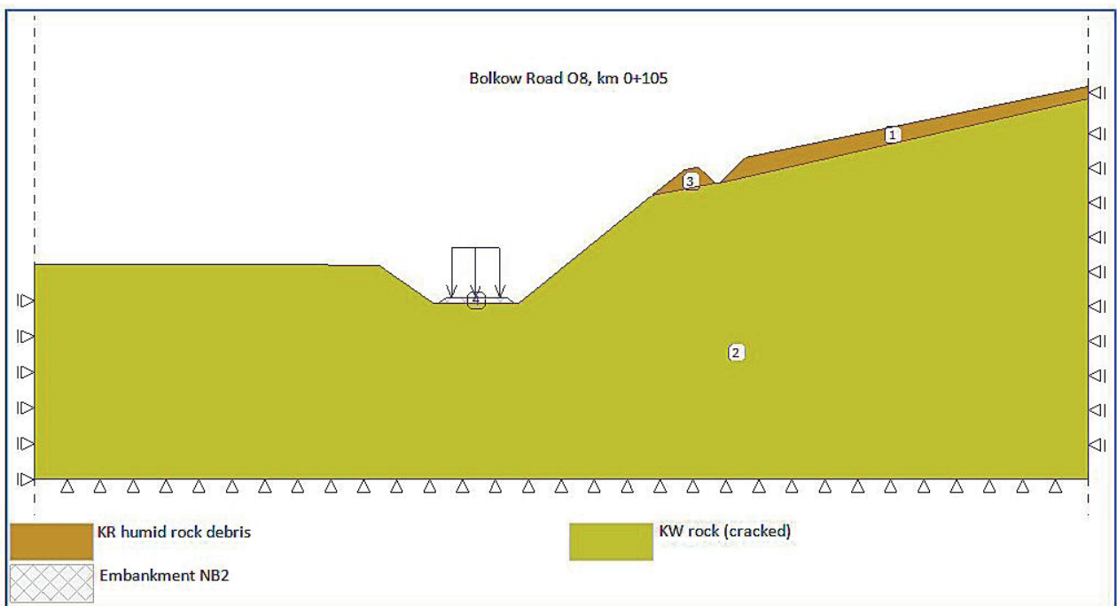
Figure 13: Designed slope profile of the road O8 excavation in the cross section of km 0 + 105.00
